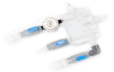
Machined Acrylic Flow Cell with magnetic flow switch
